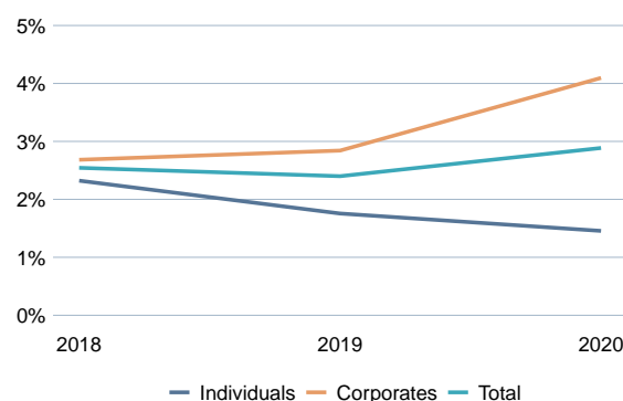
Figure 4.5: Probability of default (PD)
