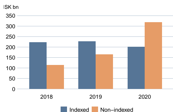
Figure 4.21: Indexed vs. non-indexed mortgages
