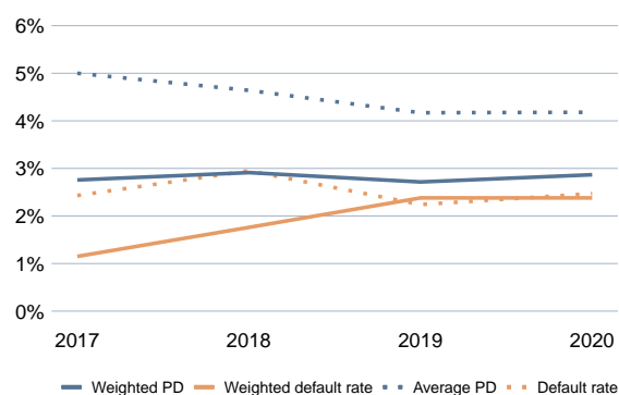
Figure 4.32: Default rate vs. PD - Individuals
