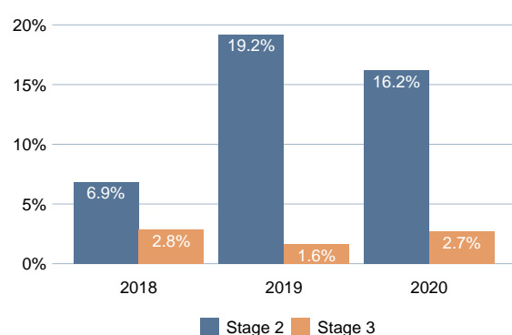
Figure 4.17: Staging - Construction companies
