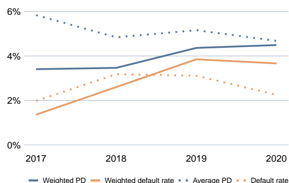
Figure 4.16: Default rate vs. PD - Construction companies
