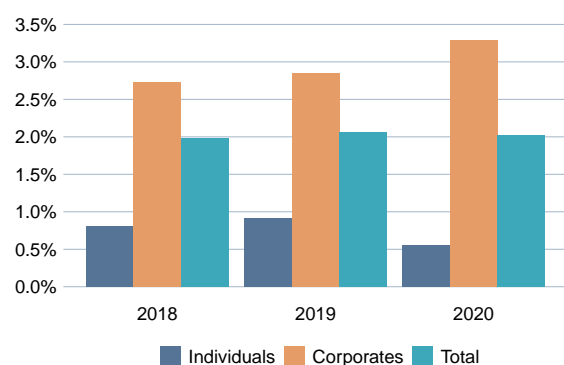
Figure 4.7: Stage 3 loans (% of total portfolio)
